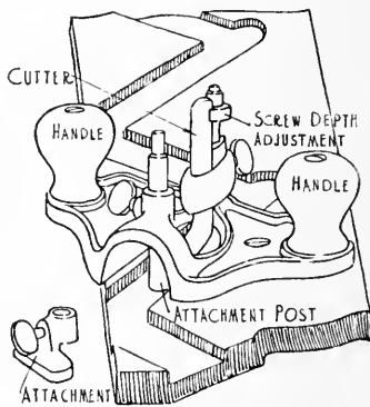
FIG. 76. ROUTER PLANE.
